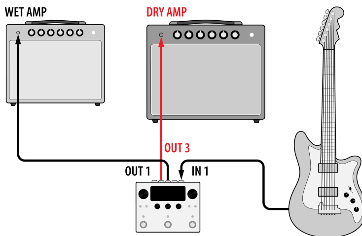
Fig. 3.6 Wet/Dry guitar amp configuration
