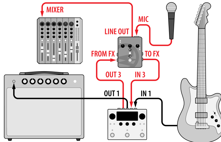
Fig. 3.10 Guitar and Vocals with MixingLink
