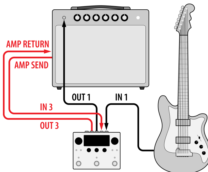
Fig. 3.11 A Pre-post or 4-cable method guitar amp configuration
