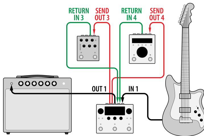
Fig. 3.3 Two Mono Inserts
