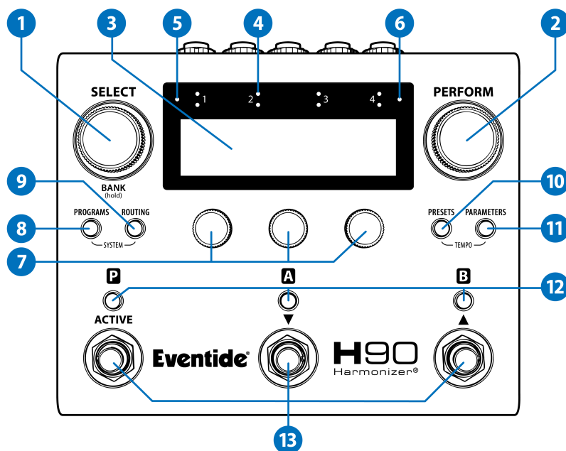
Fig. 2.1 H90 Top Panel
