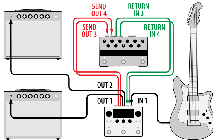
Fig. 3.4 One Stereo Insert
