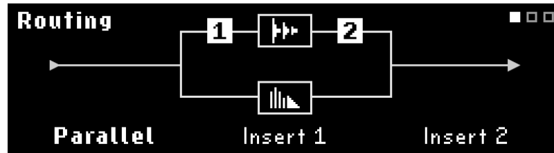
Fig. 6.11 Inserts 1 & 2 in Parallel, with Insert 1 pre-Preset A, and Insert 2 post-Preset A
