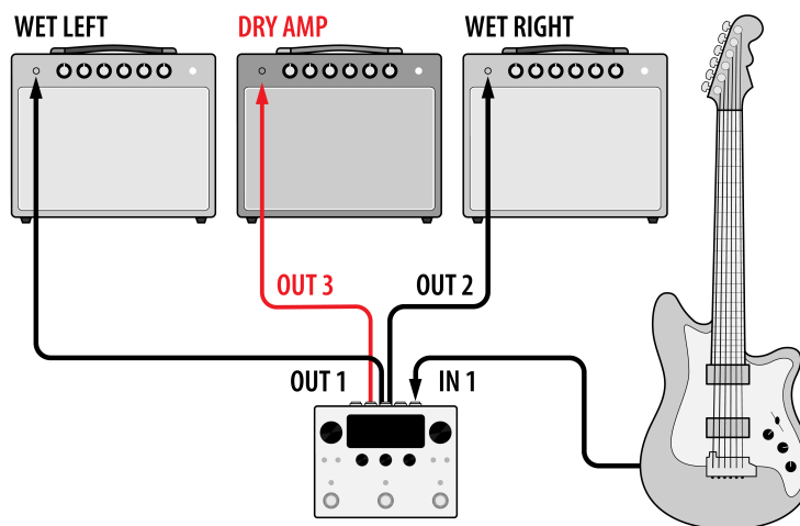
Fig. 3.9 Wet/Dry/Wet guitar amp configuration
