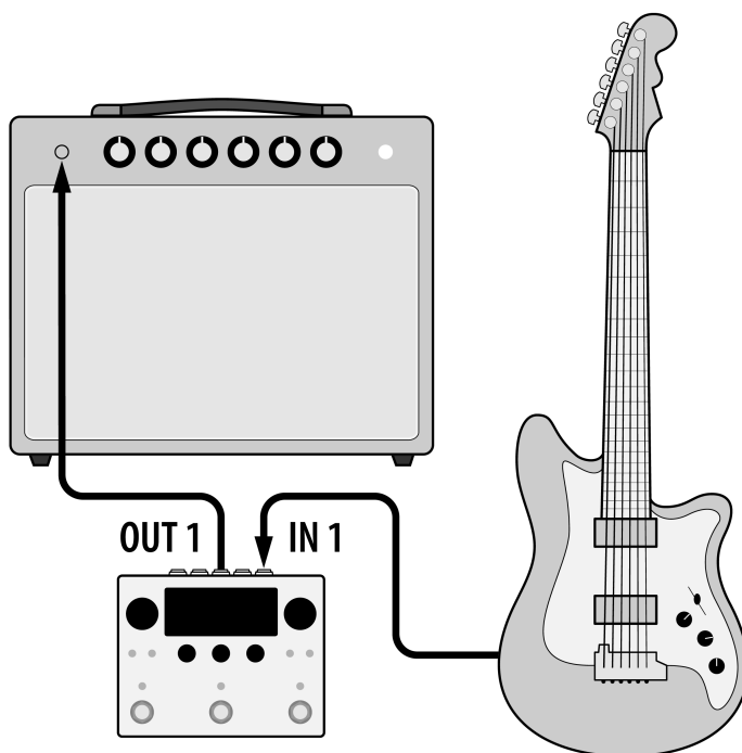
Fig. 3.2 A simple mono guitar configuration
